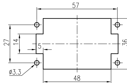
面板安装开孔图 Panel cut out
