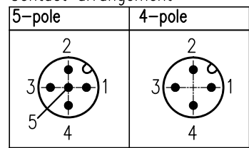
针位排布图 Contact arrangement
