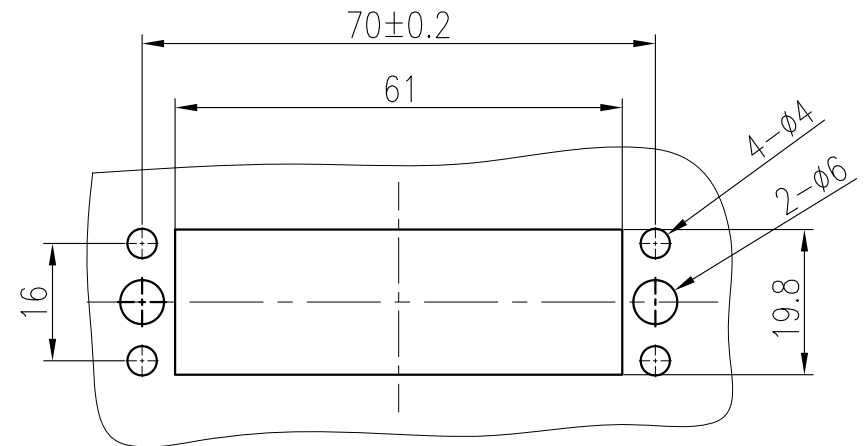
面板开孔图 Panel cut out
